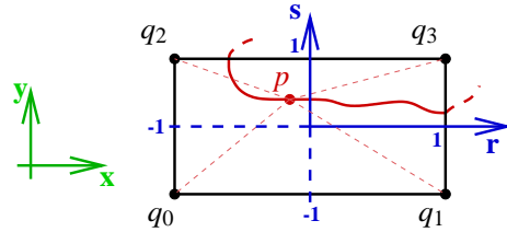
Figure 3: Interpolation of a surface vertex p inside a boundary element.
