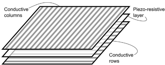
Figure 3 The three layers that constitute the TexiCare textile sensors.
