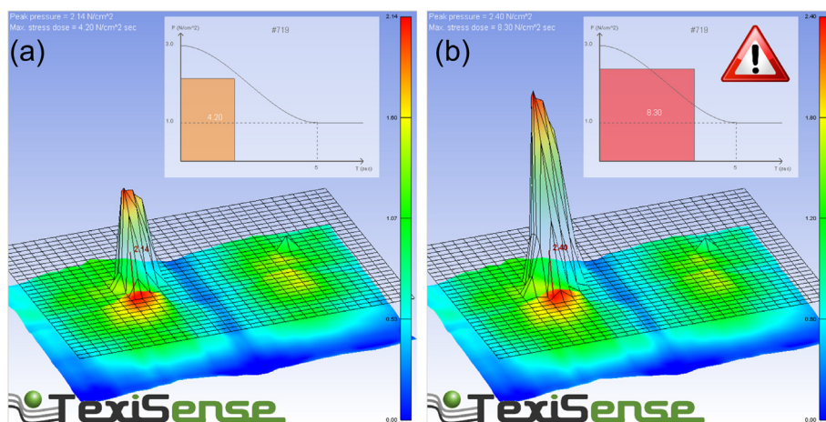
Figure 9 Accumulation of strain: a strain level applied during a short period (a) can become dangerous if it is maintained for too long (b).
