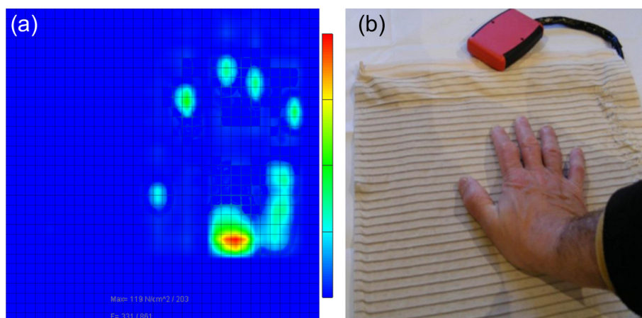
Figure 4 The 32 \times 32 TexiCare sensors textile matrix; (a) data collected from the device that reflect the pressures applied at the textile surface (b).
