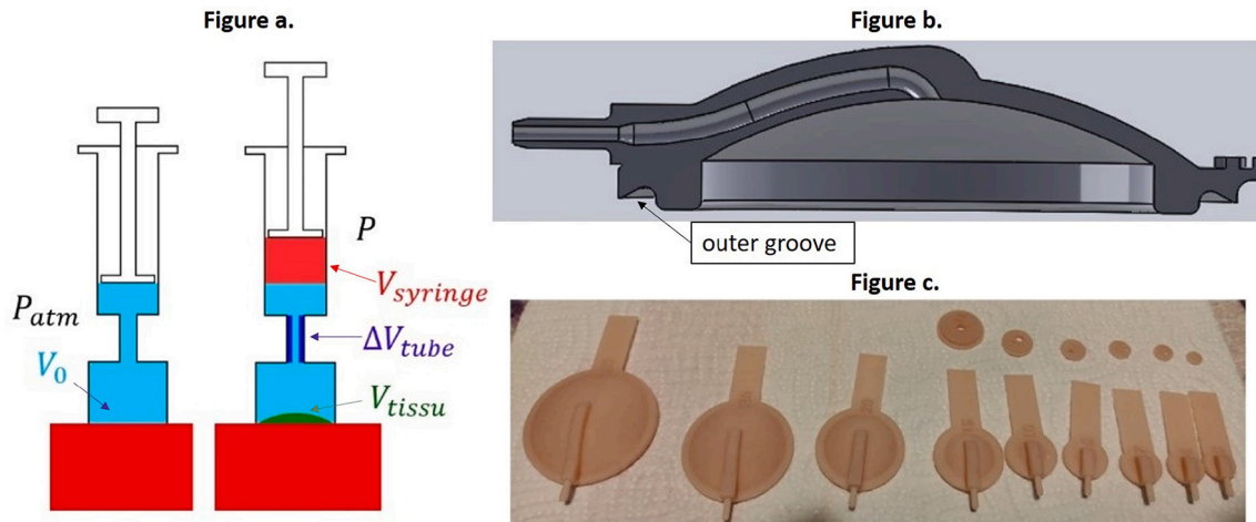
Fig. 1. VLASTIC device, with aspiration cups of various diameters; -a- functional sketch of the device -b- cross-section of a cup -c- all the different cup diameters available (from 30 mm to 4 mm).
