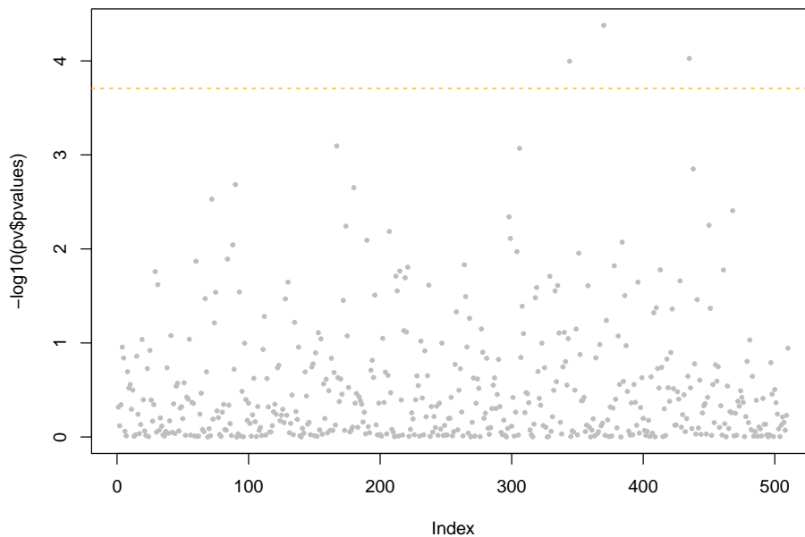
Figure 7: Offset example: p -values for LFMM2 tests.
