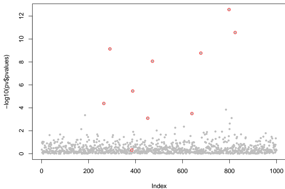
Figure 8: Manhattan plot of \log_{10} p -values for LFMM2 tests. The loci showing real associations are circled in red.
