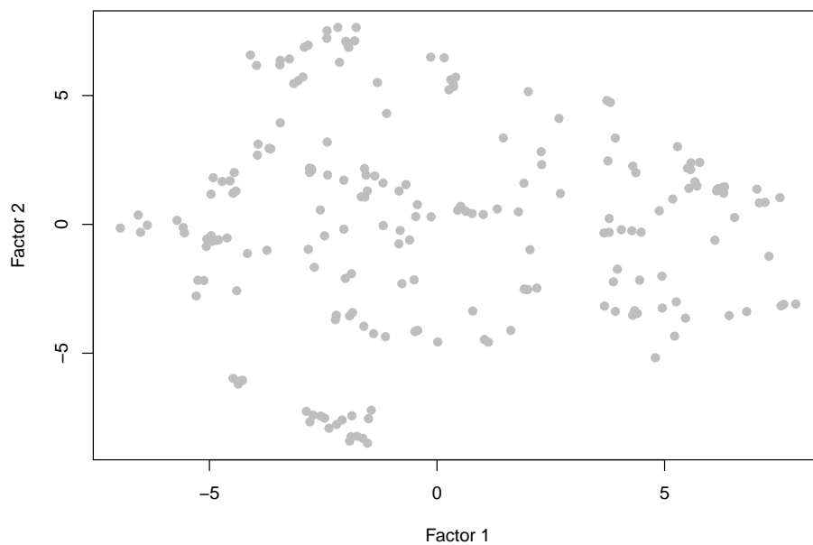
Figure 6: Latent factors estimated in the offset example data analysis.
